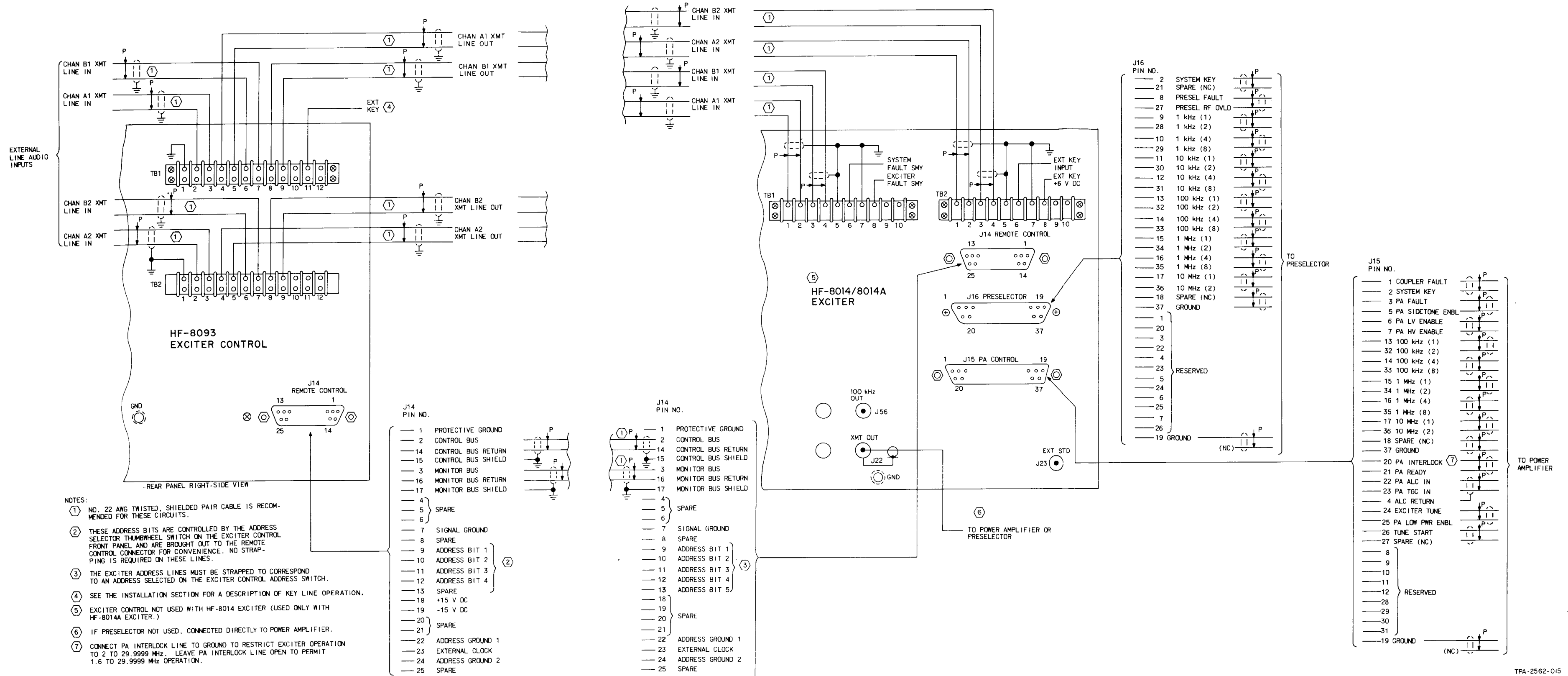
HF-8014( ) Exciter, Typical Installation Figure 6
