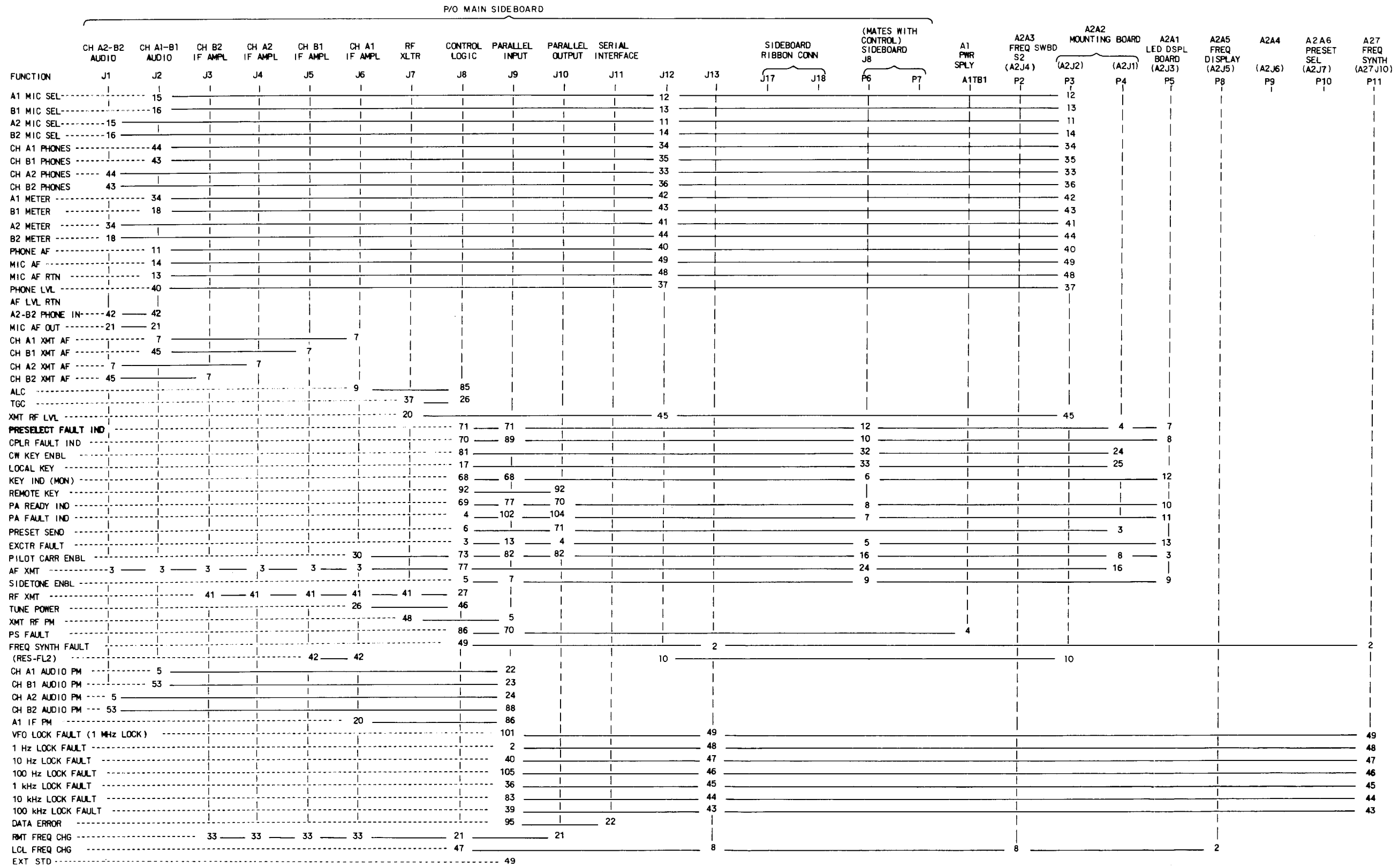
Chassis, Main Sideboard and Ribbon Cabling, Schematic Diagram Figure 1 (Sheet 1 of 6)
