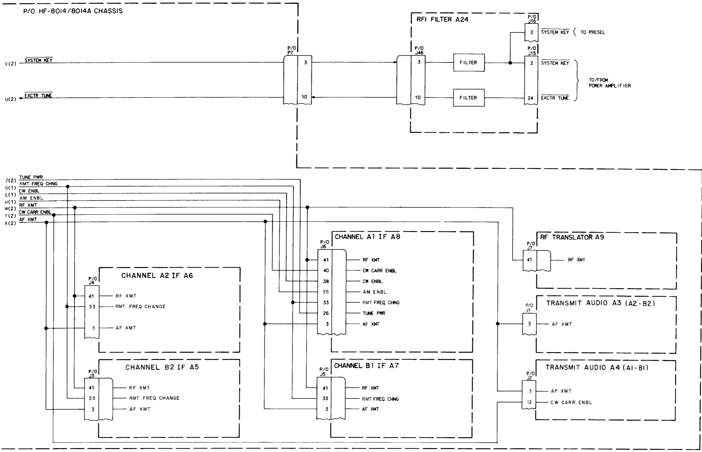
Key and Carrier Control Functions, Block Diagram Figure 5 (Sheet 3)
