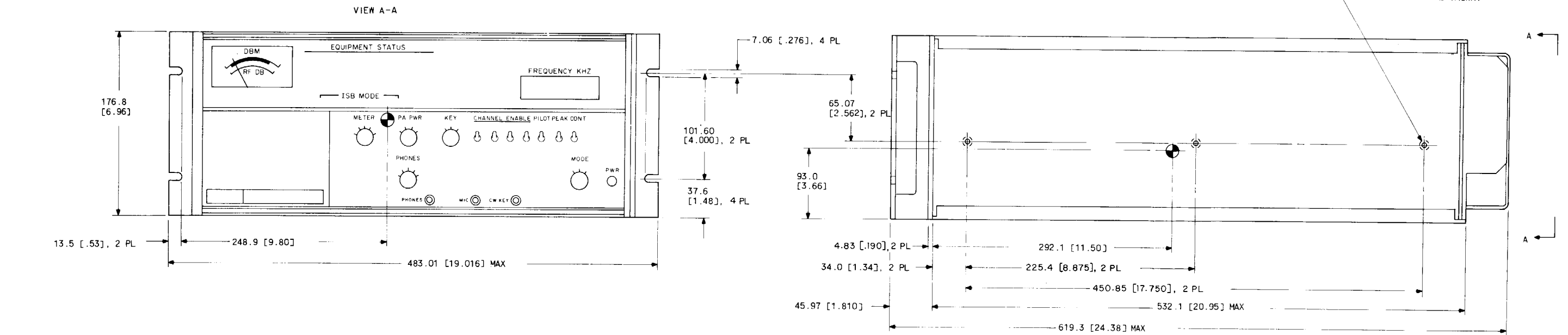
HF-8014( ) Exciter, Outline and Mounting Dimensions Figure 7
